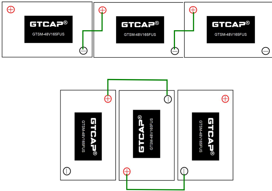
Figure 1, possible series connection of 48V modules
